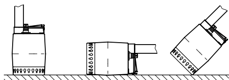
Fig. 10 Pumpestillinger
