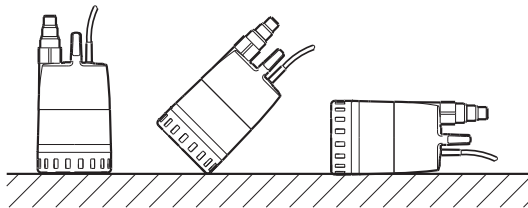
Fig. 2 Pumpestillinger
