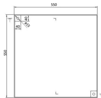
Type 2-50 & 2-70
