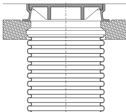
Cast iron chamber cover 600 Load bearing concrete ring 600
